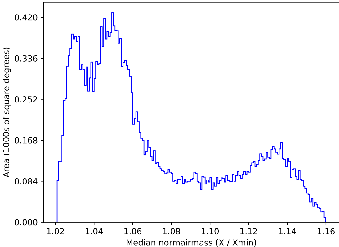
reweight_plane_v3.3_10yrs All sky all bands: Median normairmass
