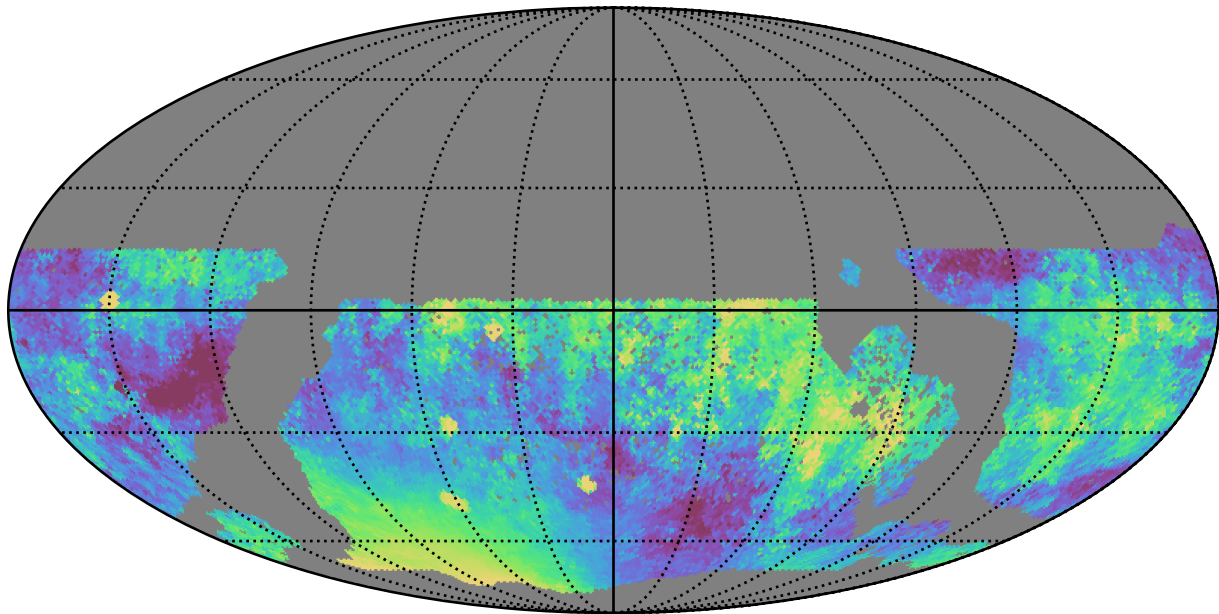
reweight_plane_v3.3_10yrs WFD z band: Median moonDistance
