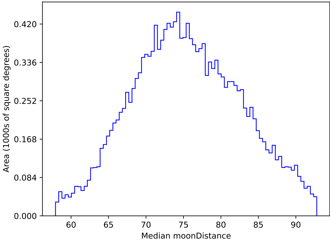
reweight_plane_v3.3_10yrs WFD z band: Median moonDistance
