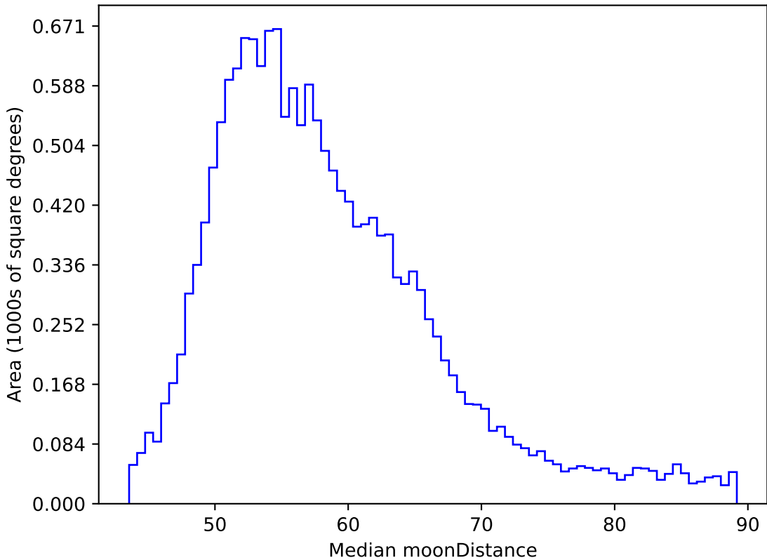
reweight_plane_v3.3_10yrs WFD y band: Median moonDistance
