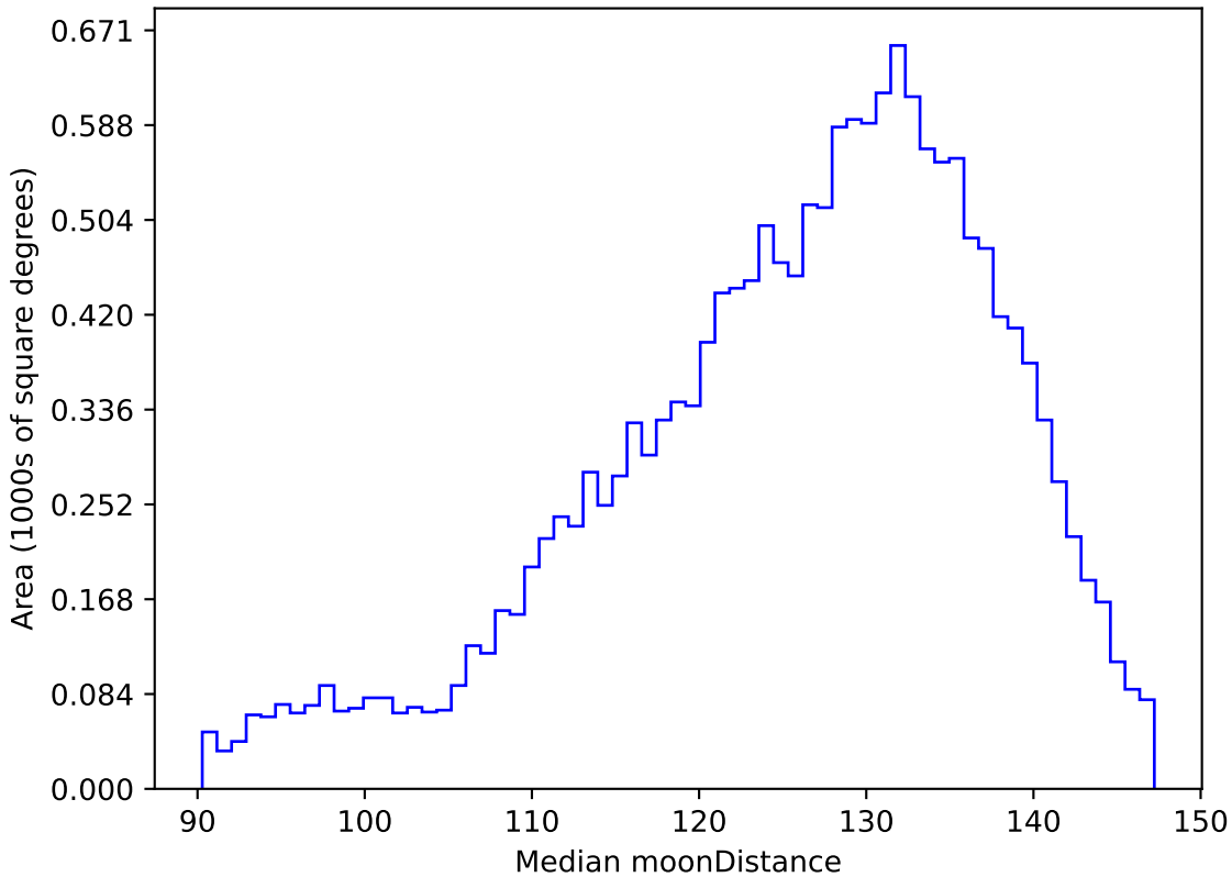
reweight_plane_v3.3_10yrs WFD u band: Median moonDistance
