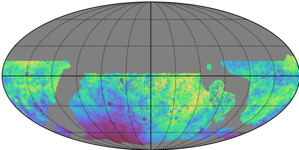
reweight_plane_v3.3_10yrs WFD r band: Median moonDistance
