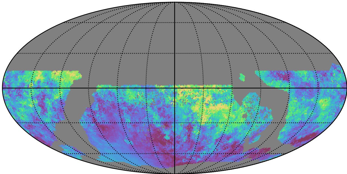
reweight_plane_v3.3_10yrs WFD i band: Median moonDistance
