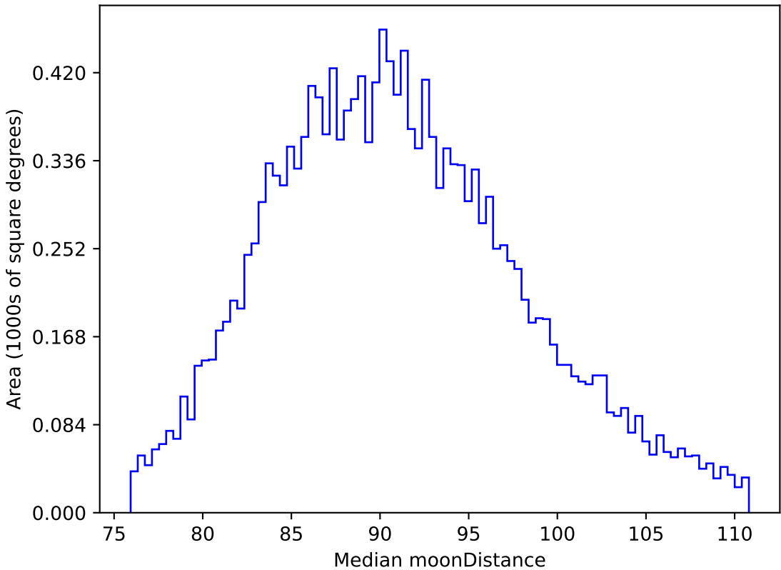
reweight_plane_v3.3_10yrs WFD i band: Median moonDistance
