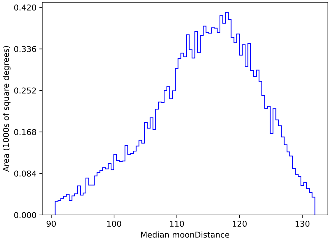
reweight_plane_v3.3_10yrs WFD g band: Median moonDistance
