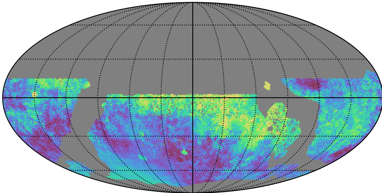
reweight_plane_v3.3_10yrs WFD all bands: Median moonDistance
