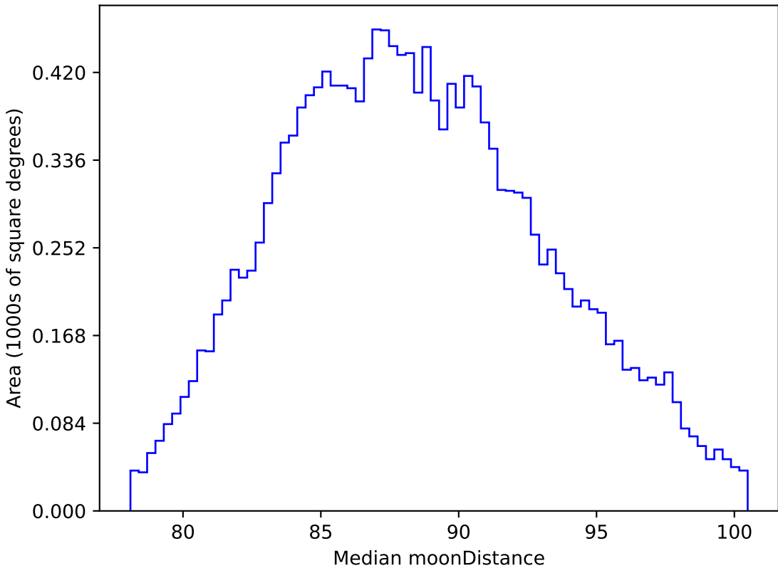
reweight_plane_v3.3_10yrs WFD all bands: Median moonDistance
