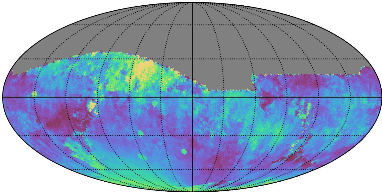
reweight_plane_v3.3_10yrs All sky z band: Median moonDistance
