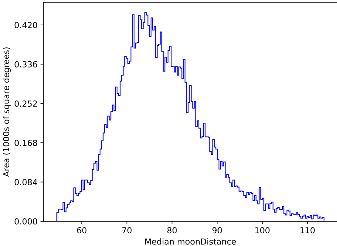
reweight_plane_v3.3_10yrs All sky z band: Median moonDistance
