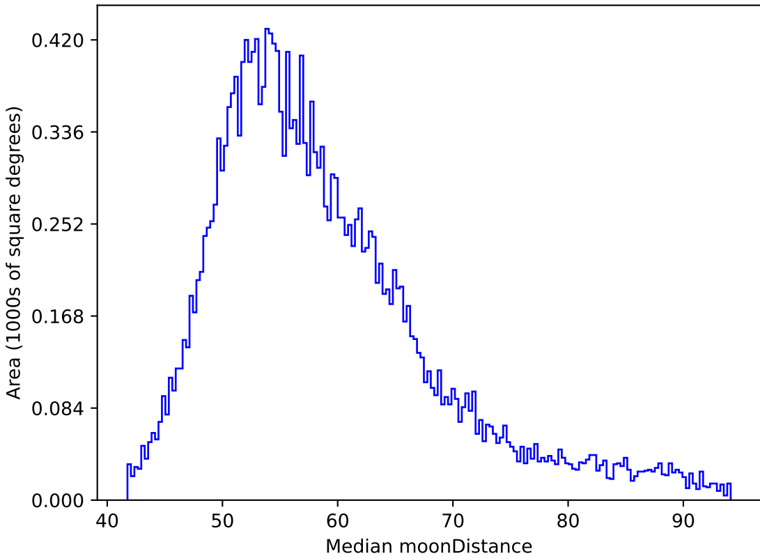
reweight_plane_v3.3_10yrs All sky y band: Median moonDistance
