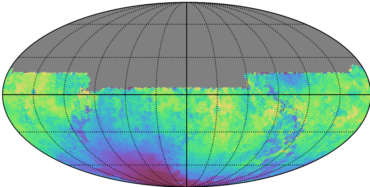
reweight_plane_v3.3_10yrs All sky u band: Median moonDistance
