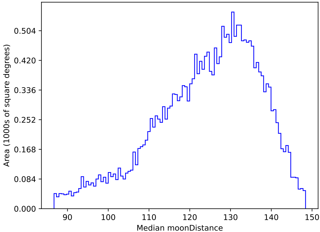
reweight_plane_v3.3_10yrs All sky u band: Median moonDistance
