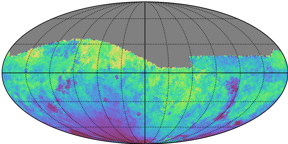
reweight_plane_v3.3_10yrs All sky r band: Median moonDistance
