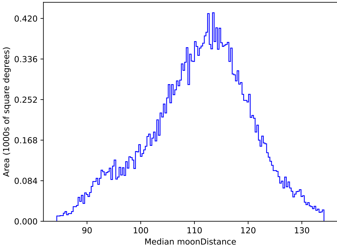
reweight_plane_v3.3_10yrs All sky r band: Median moonDistance
