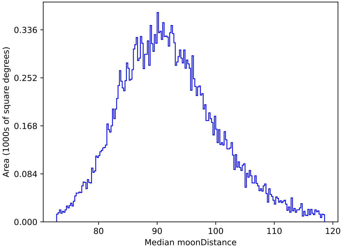
reweight_plane_v3.3_10yrs All sky i band: Median moonDistance
