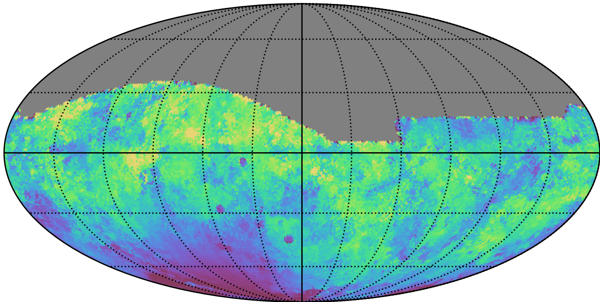
reweight_plane_v3.3_10yrs All sky g band: Median moonDistance
