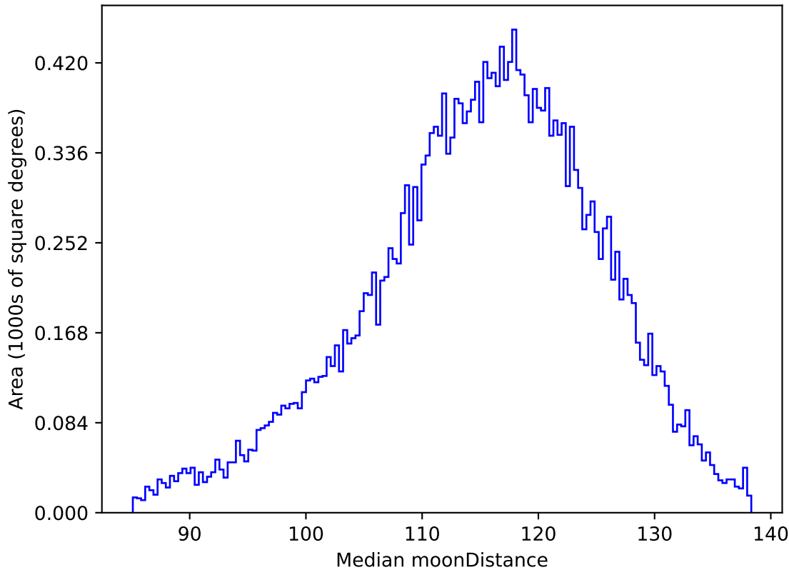
reweight_plane_v3.3_10yrs All sky g band: Median moonDistance
