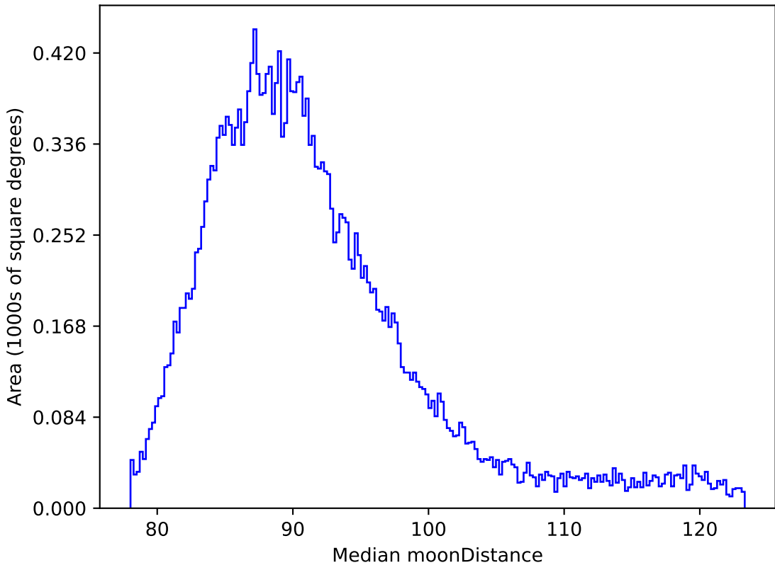
reweight_plane_v3.3_10yrs All sky all bands: Median moonDistance
