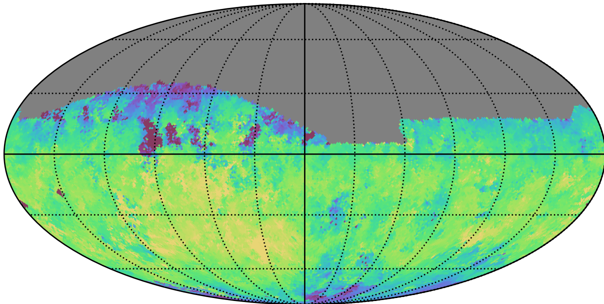
reweight_plane_v3.3_10yrs Yr 1 z band: Median fiveSigmaDepth
