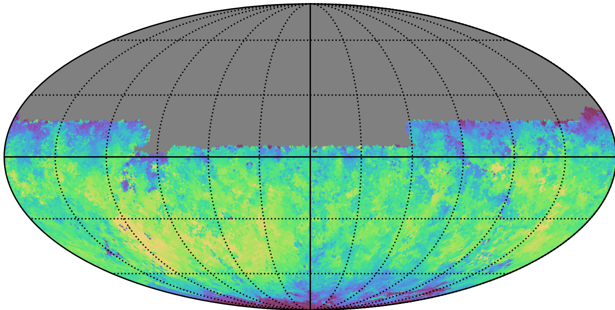
reweight_plane_v3.3_10yrs Yr 1 y band: Median fiveSigmaDepth
