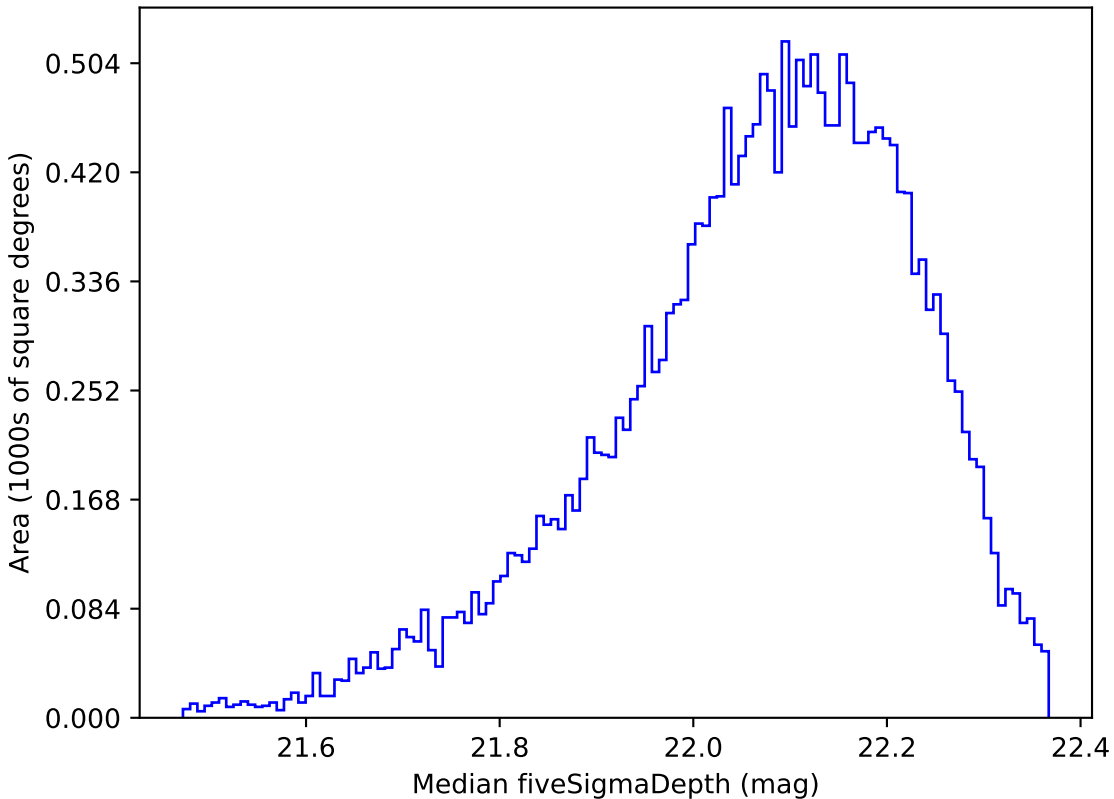
reweight_plane_v3.3_10yrs Yr 1 y band: Median fiveSigmaDepth
