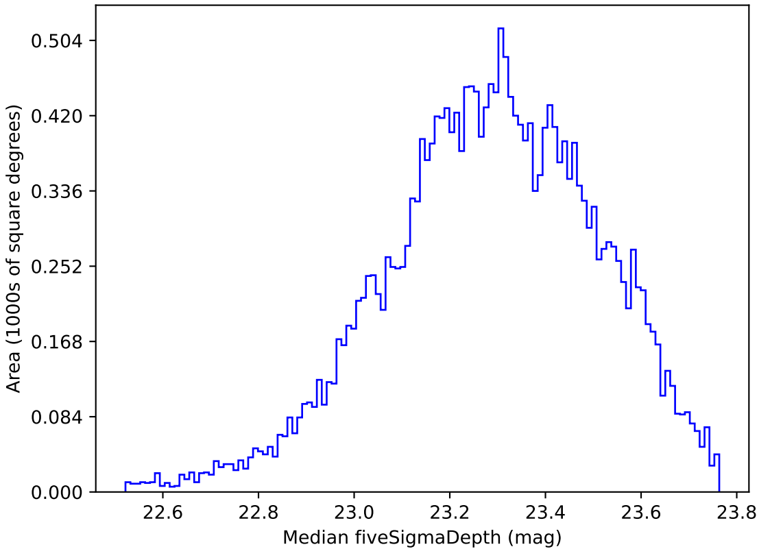
reweight_plane_v3.3_10yrs Yr 1 u band: Median fiveSigmaDepth
