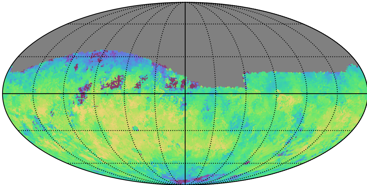
reweight_plane_v3.3_10yrs Yr 1 r band: Median fiveSigmaDepth
