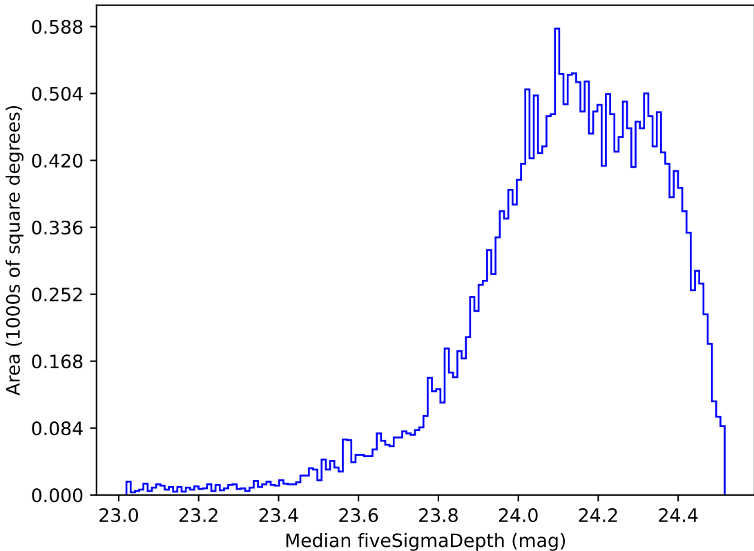
reweight_plane_v3.3_10yrs Yr 1 r band: Median fiveSigmaDepth
