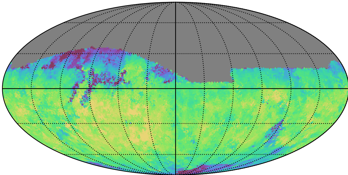
reweight_plane_v3.3_10yrs Yr 1 i band: Median fiveSigmaDepth
