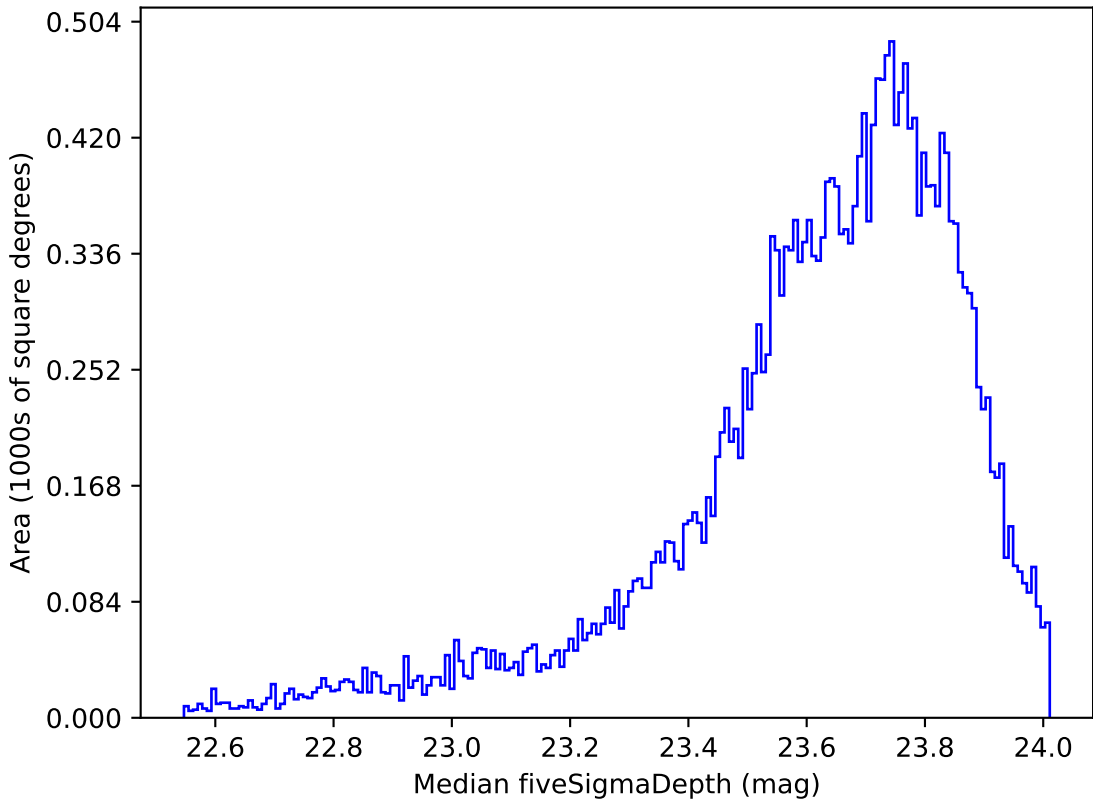
reweight_plane_v3.3_10yrs Yr 1 i band: Median fiveSigmaDepth
