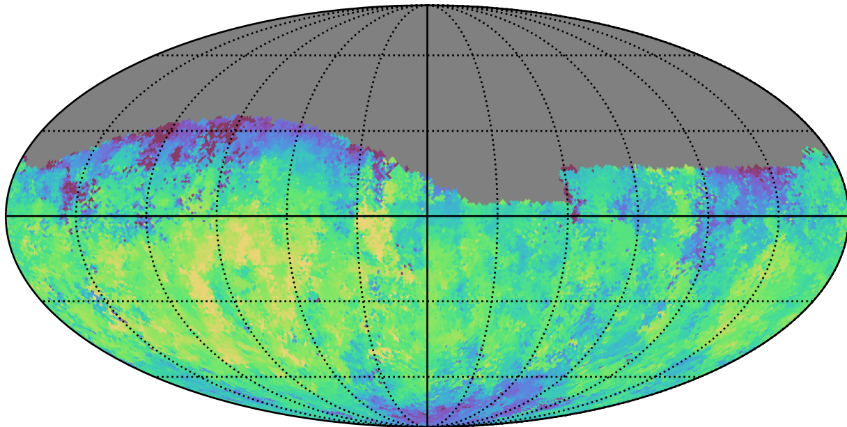
reweight_plane_v3.3_10yrs Yr 1 g band: Median fiveSigmaDepth
