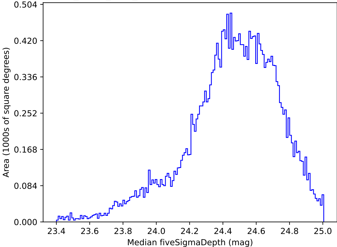
reweight_plane_v3.3_10yrs Yr 1 g band: Median fiveSigmaDepth
