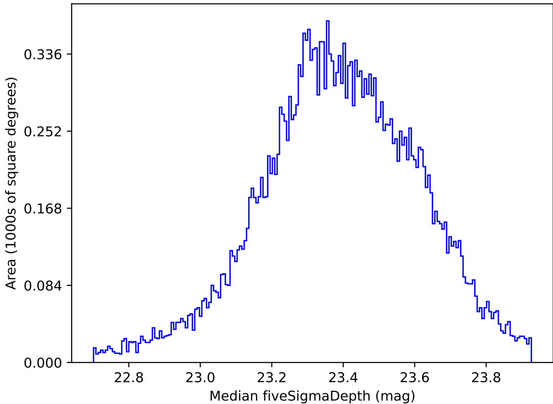
reweight_plane_v3.3_10yrs Yr 1 all bands: Median fiveSigmaDepth
