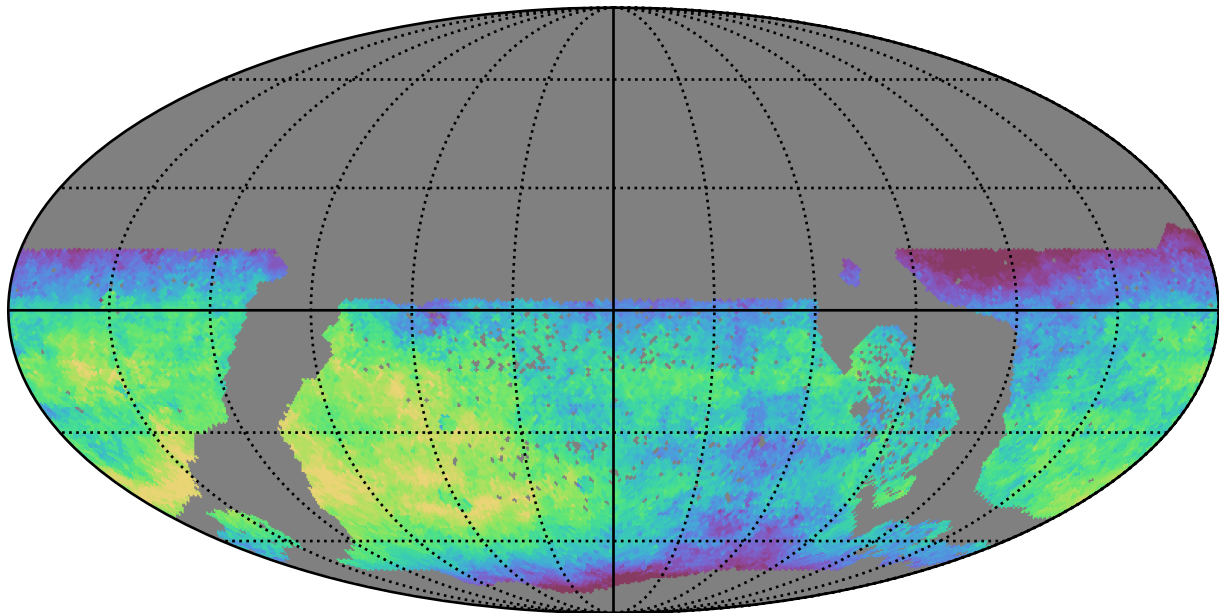
reweight_plane_v3.3_10yrs WFD z band: Median fiveSigmaDepth
