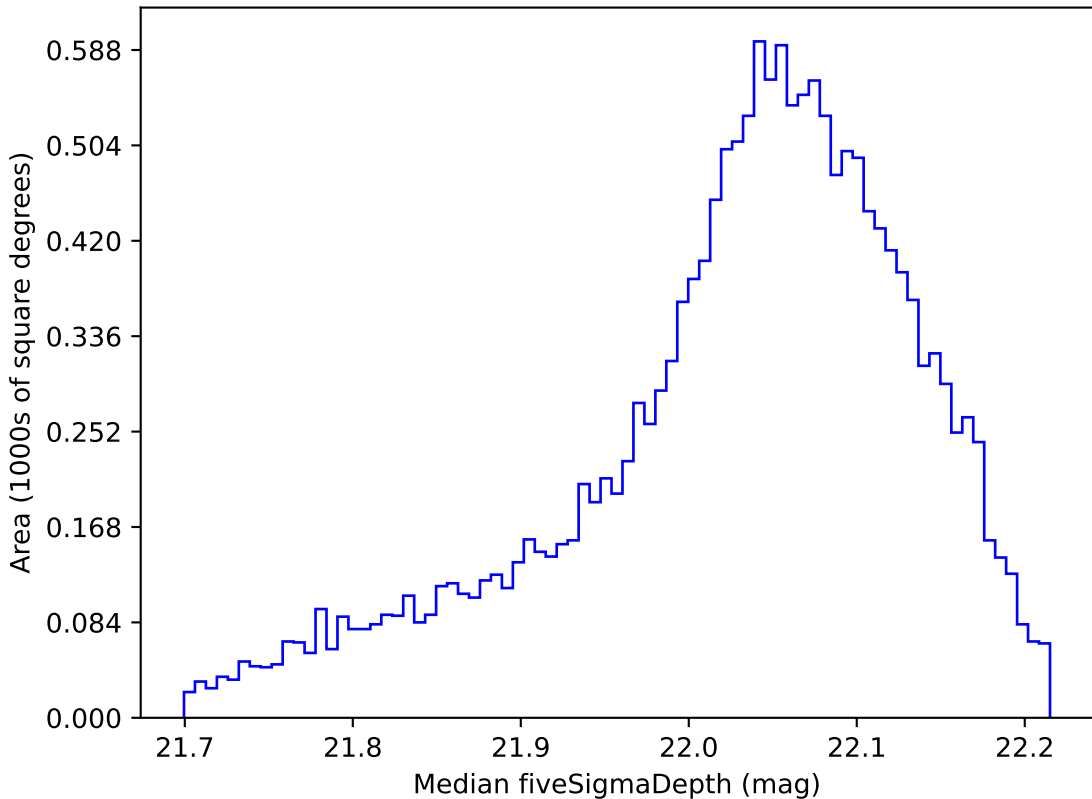
reweight_plane_v3.3_10yrs WFD y band: Median fiveSigmaDepth
