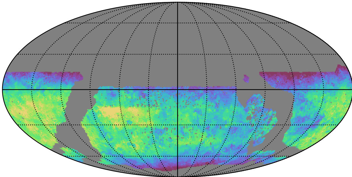
reweight_plane_v3.3_10yrs WFD u band: Median fiveSigmaDepth
