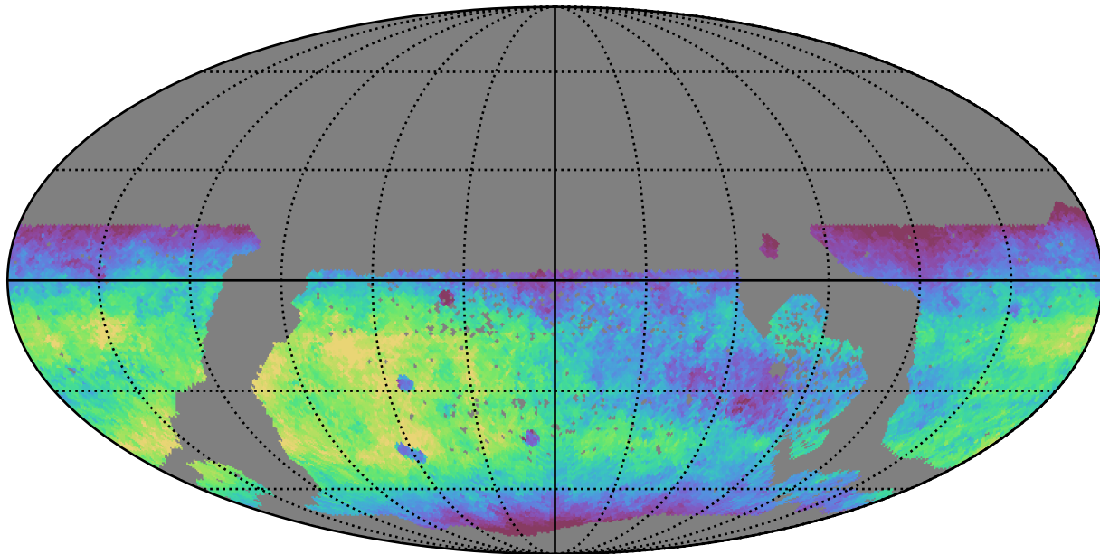
reweight_plane_v3.3_10yrs WFD r band: Median fiveSigmaDepth
