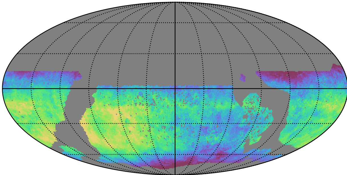
reweight_plane_v3.3_10yrs WFD i band: Median fiveSigmaDepth
