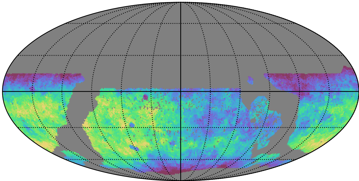
reweight_plane_v3.3_10yrs WFD g band: Median fiveSigmaDepth
