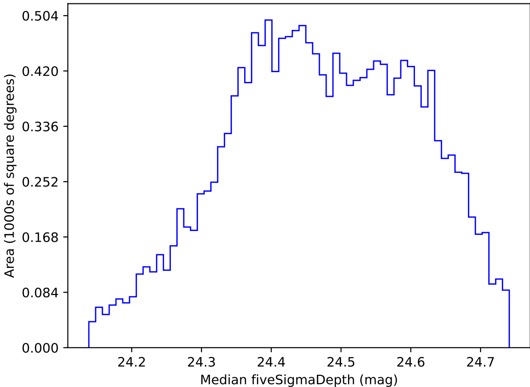
reweight_plane_v3.3_10yrs WFD g band: Median fiveSigmaDepth
