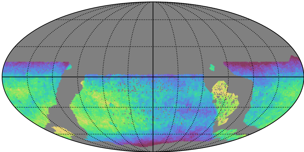
reweight_plane_v3.3_10yrs WFD all bands: Median fiveSigmaDepth
