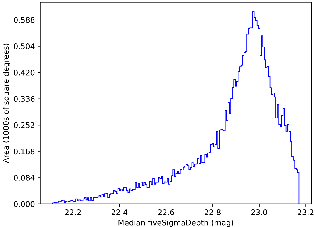
reweight_plane_v3.3_10yrs All sky z band: Median fiveSigmaDepth
