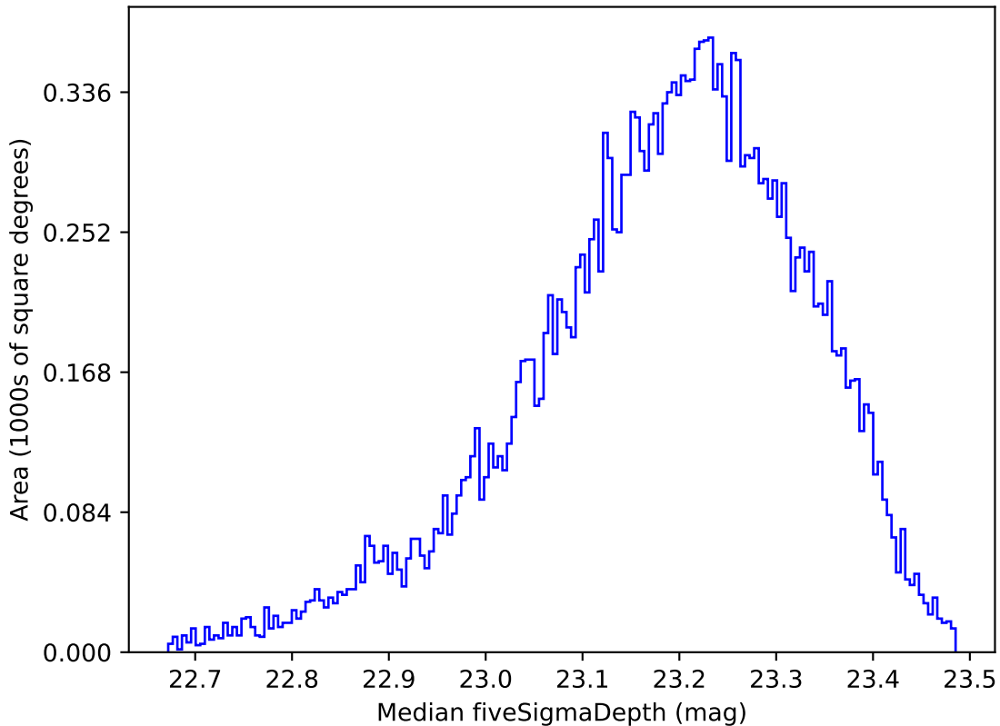
reweight_plane_v3.3_10yrs All sky u band: Median fiveSigmaDepth
