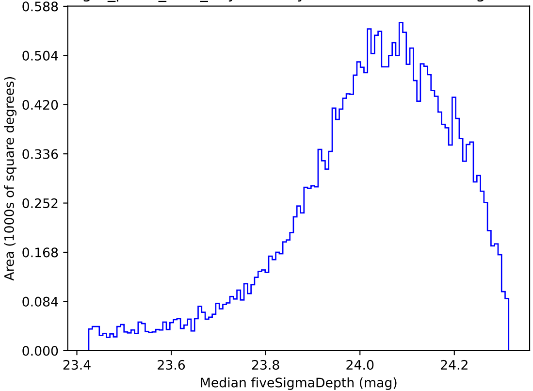
reweight_plane_v3.3_10yrs All sky r band: Median fiveSigmaDepth
