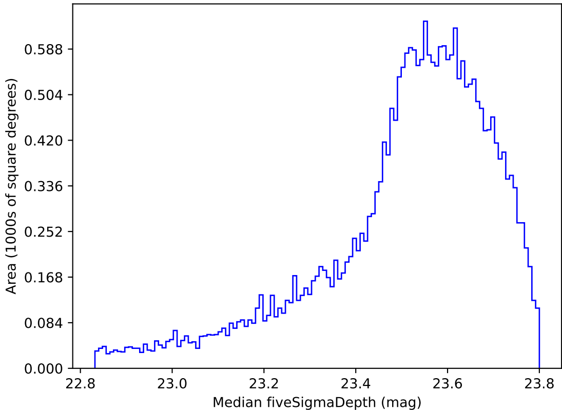
reweight_plane_v3.3_10yrs All sky i band: Median fiveSigmaDepth
