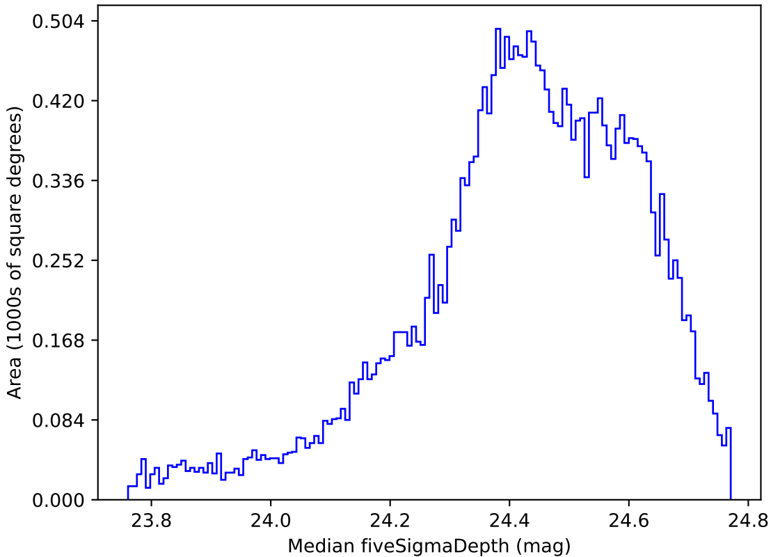
reweight_plane_v3.3_10yrs All sky g band: Median fiveSigmaDepth
