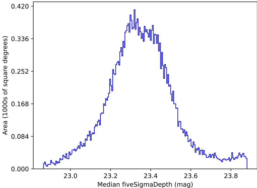
reweight_plane_v3.3_10yrs All sky all bands: Median fiveSigmaDepth
