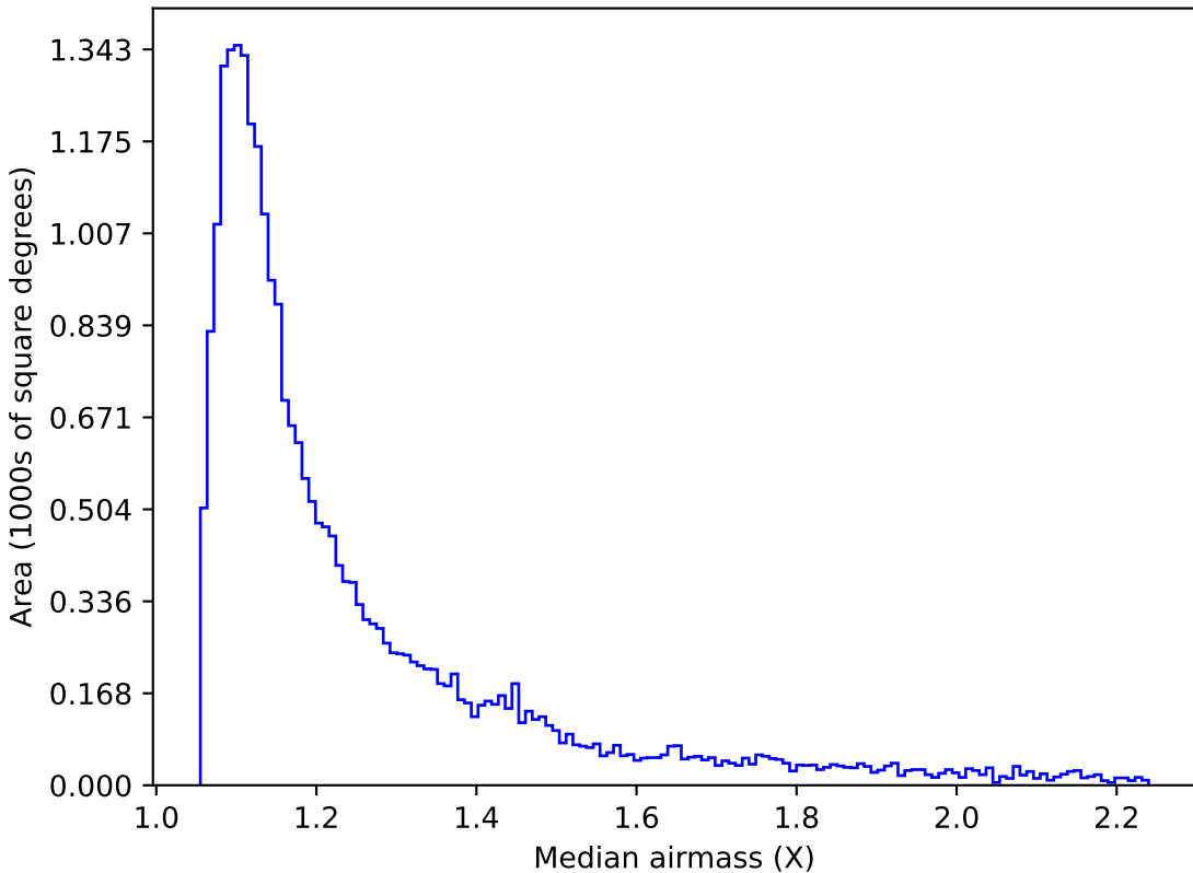
reweight_plane_v3.3_10yrs Yr 1 z band: Median airmass
