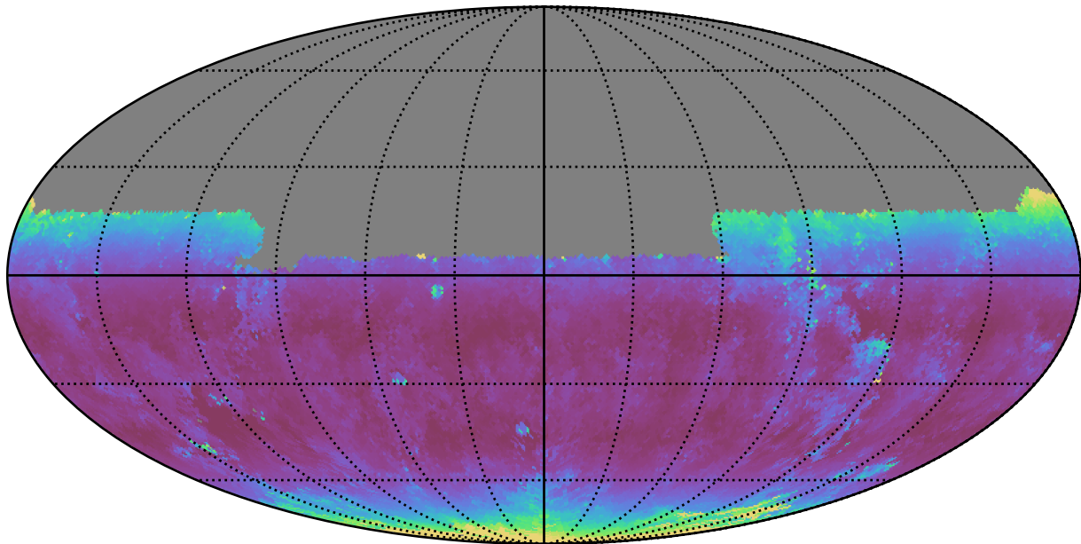
reweight_plane_v3.3_10yrs Yr 1 y band: Median airmass
