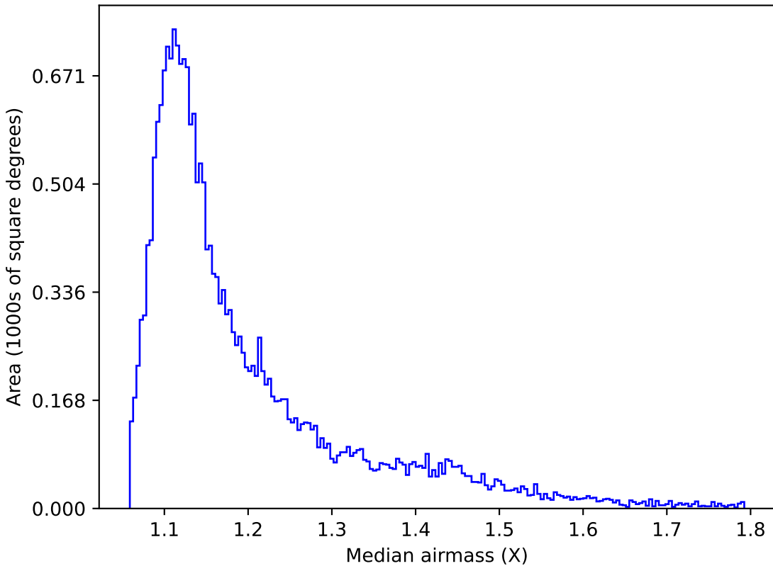
reweight_plane_v3.3_10yrs Yr 1 y band: Median airmass
